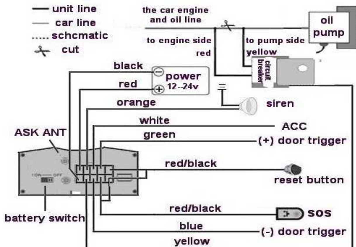
Wiring diagram
